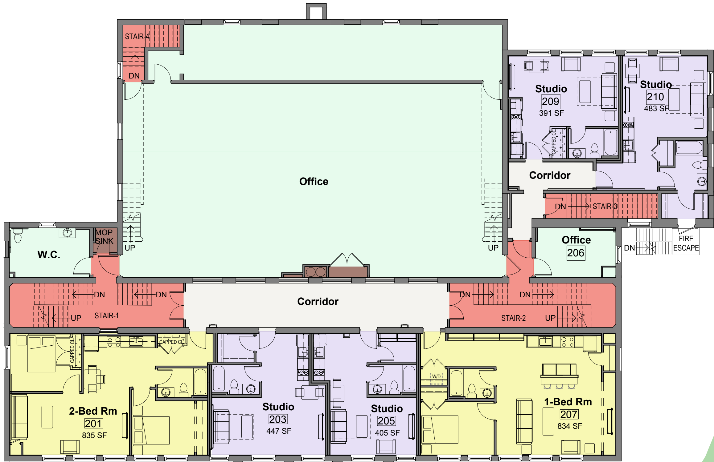
SECOND FLOOR
