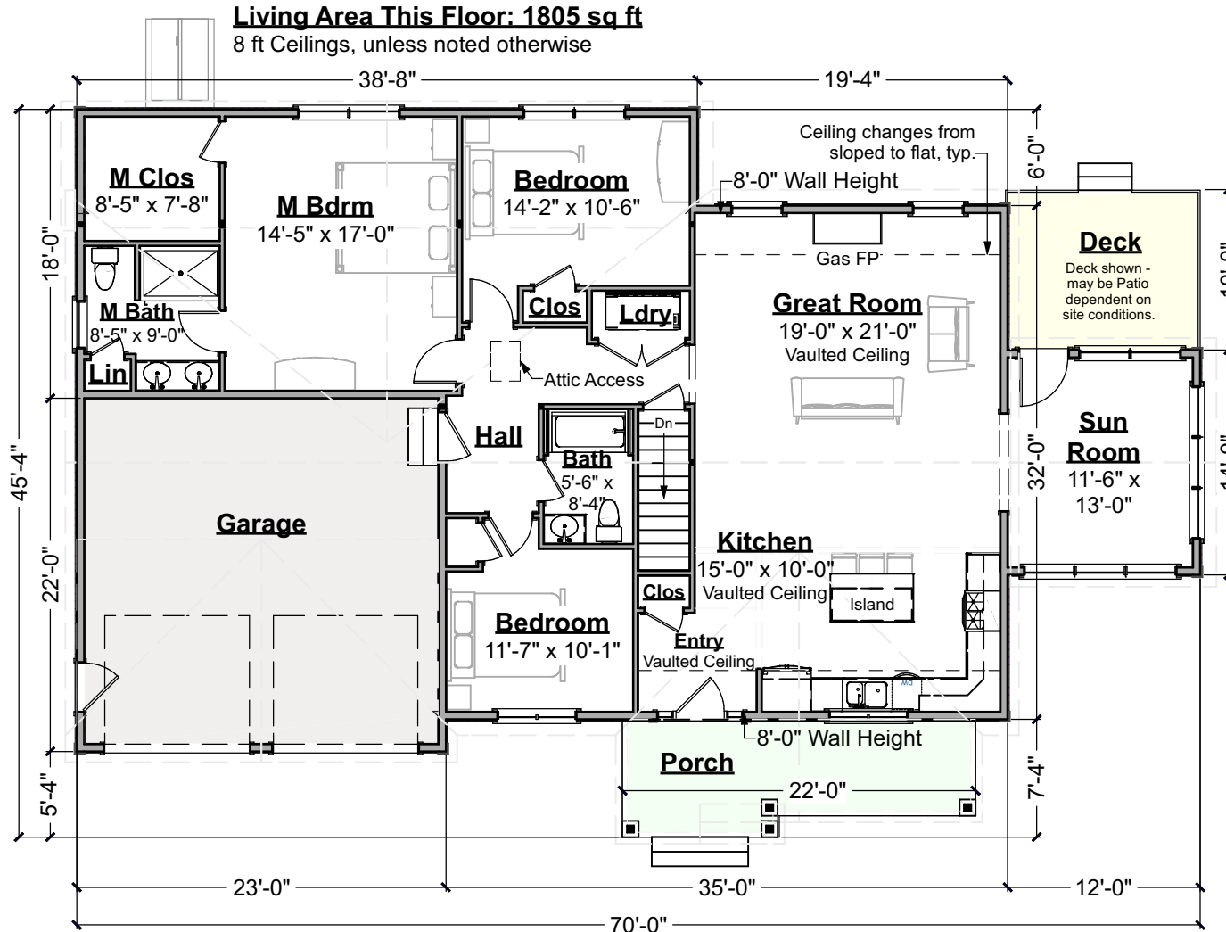
Alternate First Floor Plan - Sun Room Scale: 3/32" = 1'-0"
