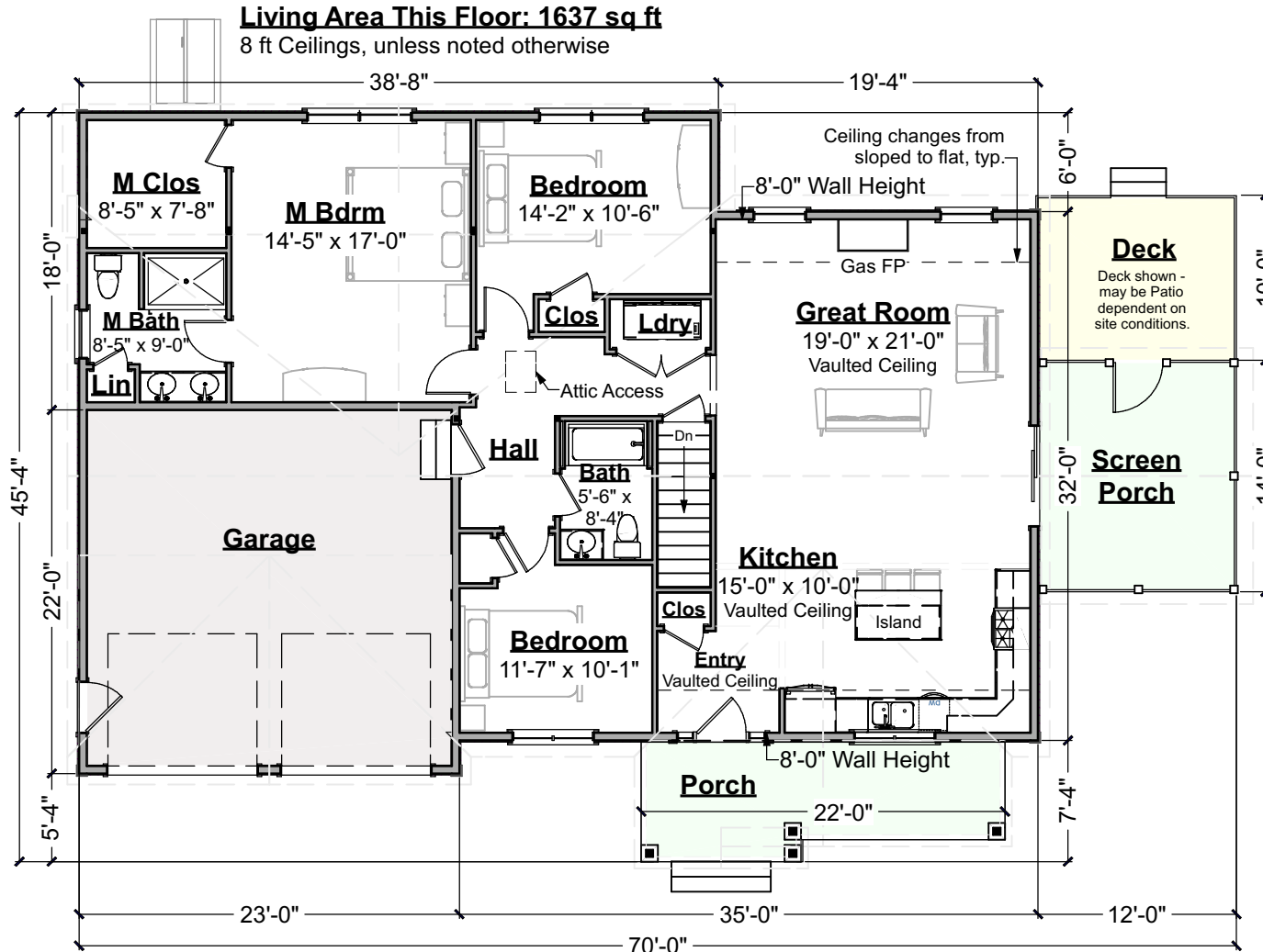
Alternate First Floor Plan - Screen Porch Scale: 3/32" = 1'-0"
