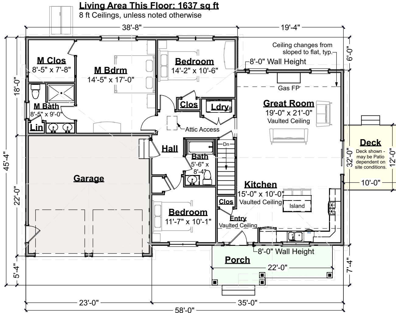
First Floor Plan Scale: 3/32" = 1'-0"
