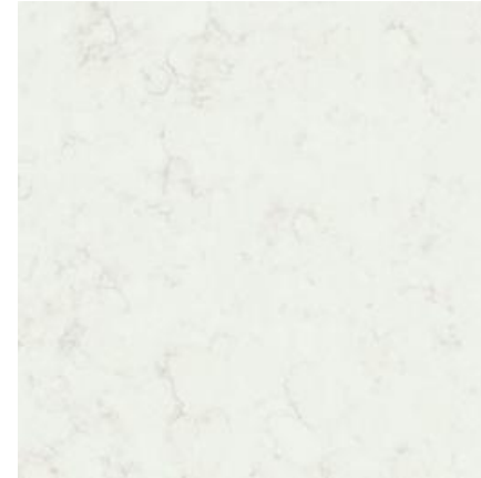
Alvarado Quartz
